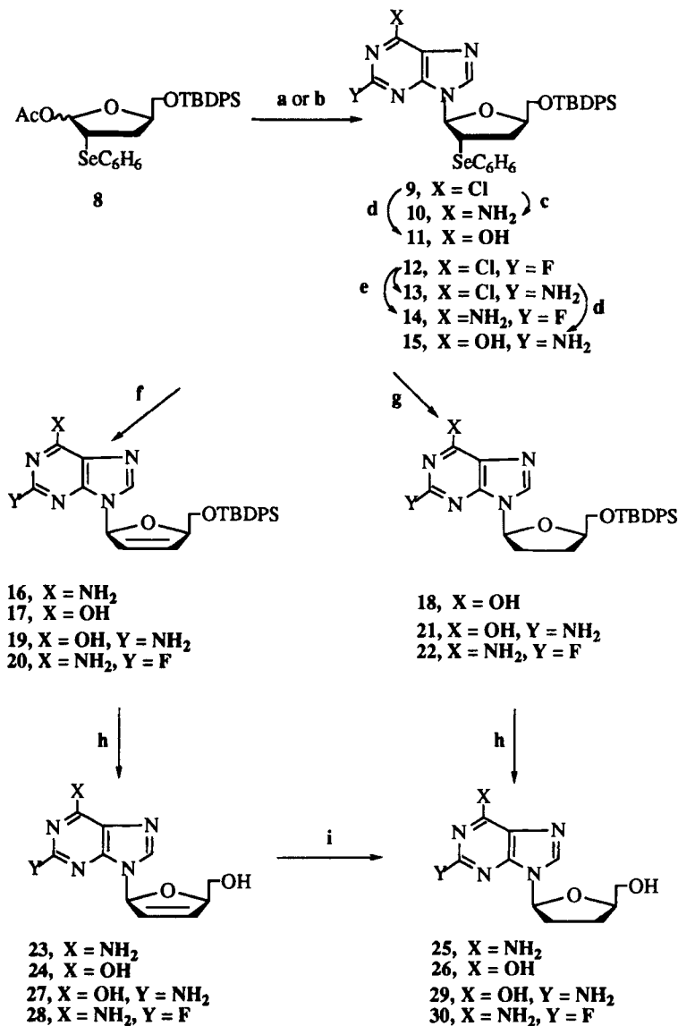
Scheme 2: Reagents and conditions: a: TMS-6-chloropurine, TMSOTf, ClCH 2 CH 2 Cl, -22 °C. b: TMS-6-chloro-2-fluoropurine, TMSOTf, ClCH 2 CH 2 Cl, 0 °C. c: NH 3 /MeOH, 80 °C. d: HSCH 2 CH 2 OH, MeOH, reflux, 24 h. e: NH 3 /DME. f: H 2 O 2 , pyridine, CH 2 Cl 2 , 0 °C. g: Bu 3 SnH, Et 3 B, benzene, rt. h: 1M TBAF/THF, rt. i: 15 psi H 2 , 10% Pd/C, rt.
