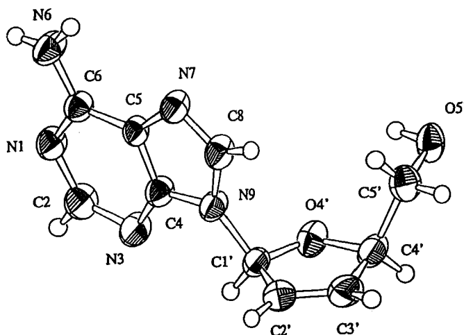
Figure 1. ORTEP Drawing of Compound 23 (L-D4A)
